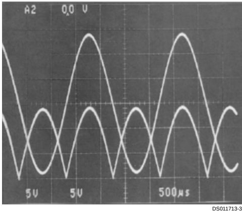
FIGURE 20. Full Wave Rectifier Waveform
